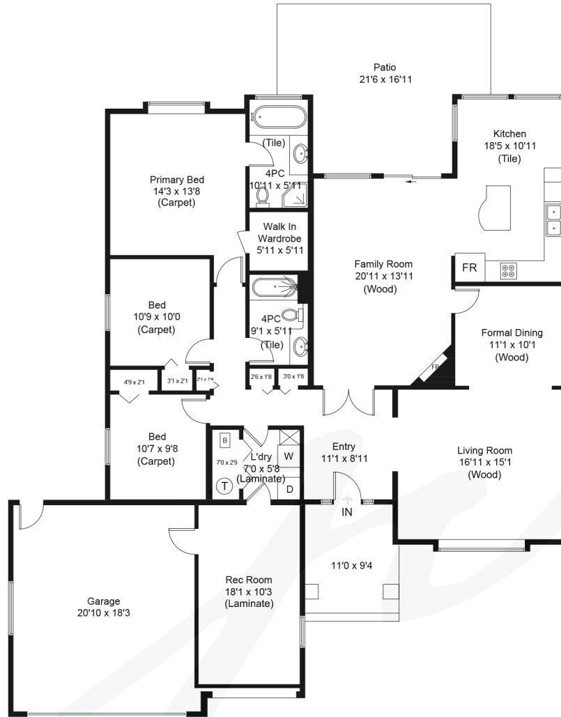
Ground Floor - 2128 sq ft
